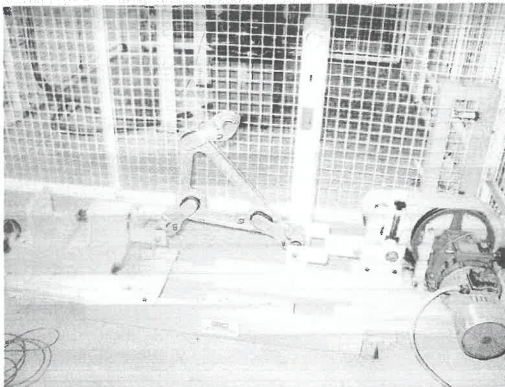
Fig. 6 – Subspan oscillation fatigue test device
