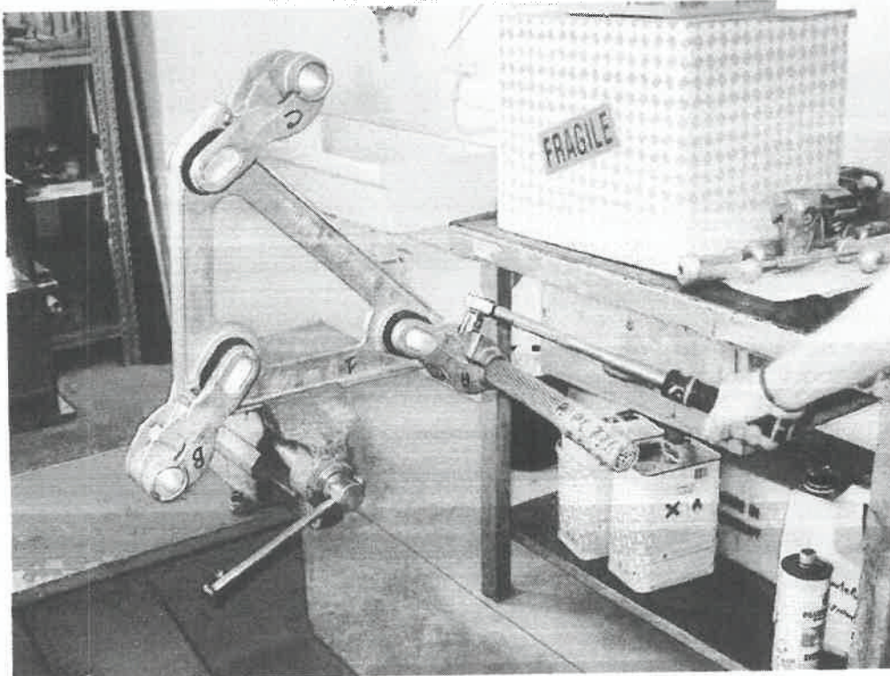
Fig. 2 – Clamp bolt tightening test
