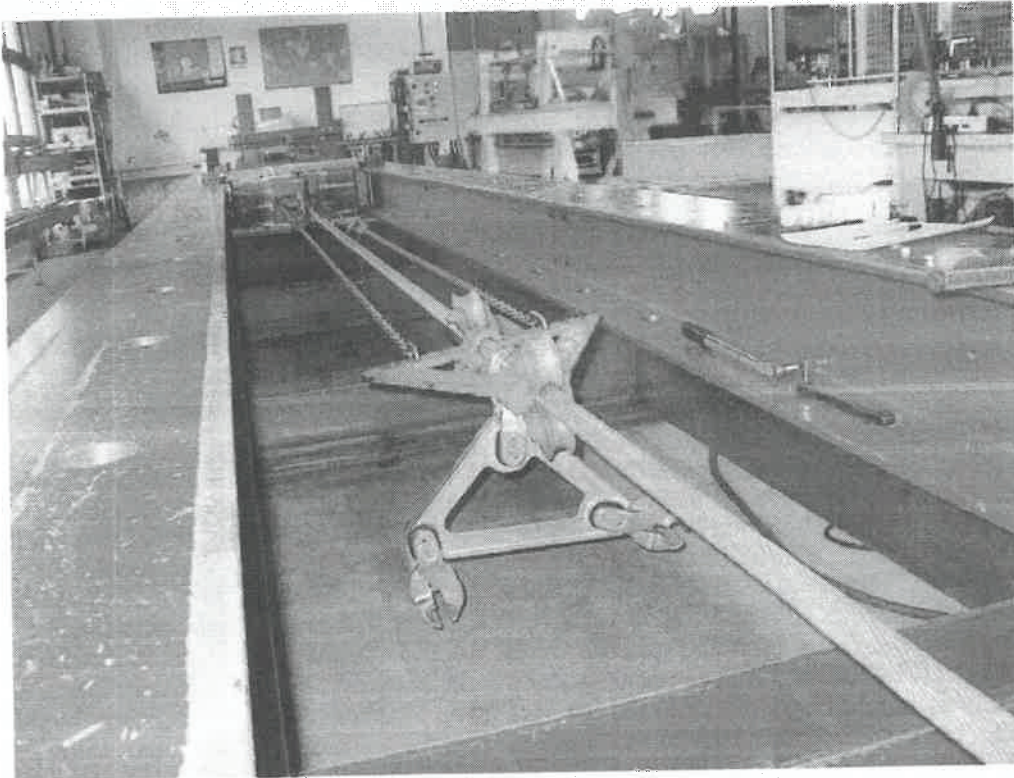
Fig. 1 – Clamp slip test device
